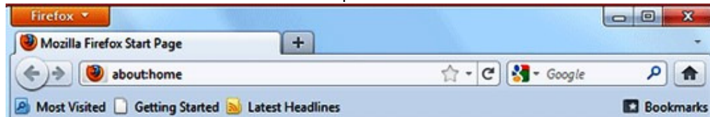
Figure 1.4 – Firefox Window
